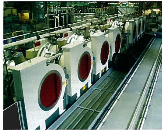
Fig. 5: Easy expanding of the modultherm-system up to 10 treatment chambers
